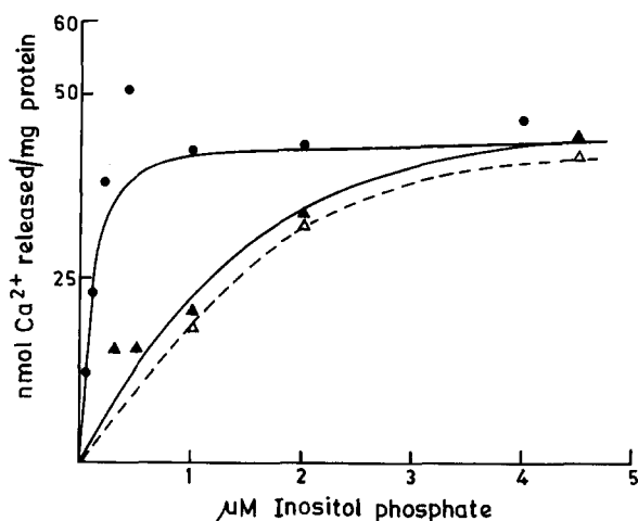
Fig. 3. Dose-dependent calcium release by Ins(1,4,5)P 3 and Ins(1,3,4,5)P 4 from permeabilized E. histolytica . Experimental details are similar to that described in Fig. 1. Data are presented as the mean of at least three experiments. ●, Ins(1,4,5)P 3 alone; ▲, Ins(1,3,4,5)P 4 alone; △, Ins(1,3,4,5)P 4 added before recovery from a saturating dose of Ins(1,4,5)P 3 .
